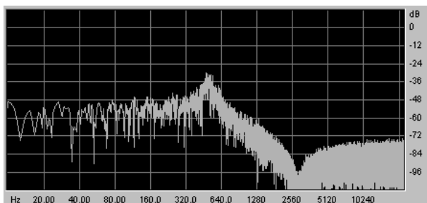
Plateau passe-bas 12 dB/octave
