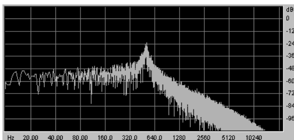
Passe-bas 12 dB/octave
