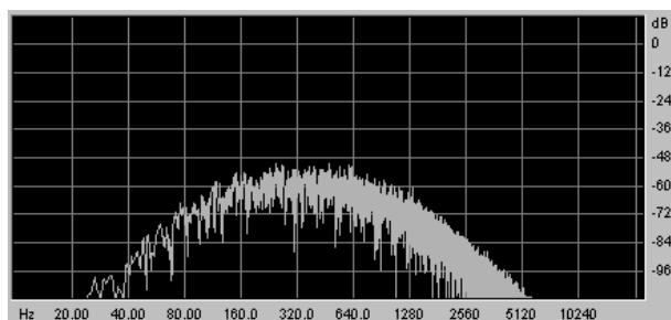
Passe-bande 24 dB/octave
