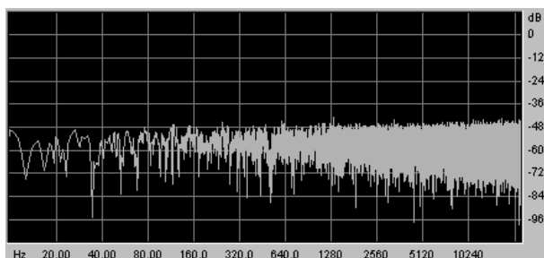
Notch 12 dB/octave
